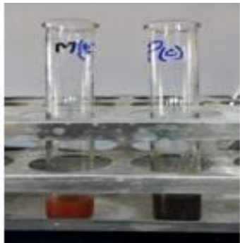
Fig 8: Amino acids
