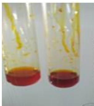
Fig 7: Steroids
